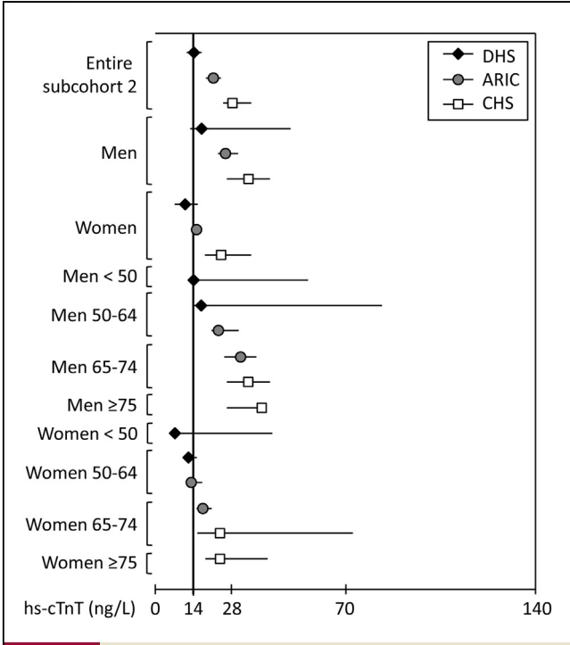
Figure 2 The 99th Percentile Values for the hs-cTnT Assay in Subcohorts 2 of the DHS, ARIC, and CHS Studies, With Further Stratification by Sex and Age Subcohorts 2 include subjects free from recent hospitalization (6 months), clinical cardiovascular disease (coronary heart disease, chronic heart failure, atrial fibrillation, prior stroke), subclinical cardiovascular disease (left ventricular hypertrophy or left ventricular ejection fraction <55% by echo or magnetic resonance imaging, left ventricular hypertrophy by electrocardiography, NT-proBNP >450 pg/ml), and stage III or greater chronic kidney disease (estimated glomerular filtration rate <60 cc/min/1.73m 2 ). Whiskers represent 95% confidence intervals. Abbreviations as in Figure 1.
